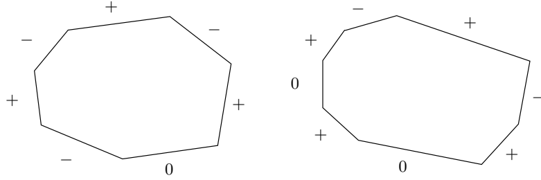
Two different examples of essential faces
